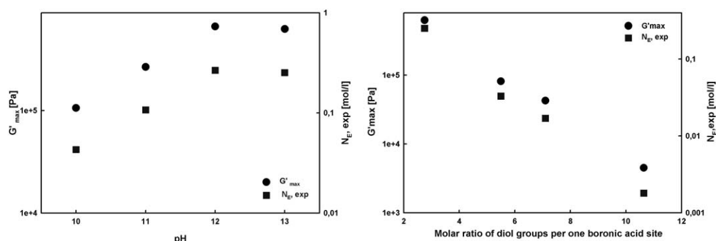
FIGURE 4 Maximum storage modulus, G'_{\max}(\omega) (circles) and the experimental number density of elastically effective network chains, N_{E, \exp} (squares), of hydrogels as a function of (a) pH at diol to boronic acid site molar ratio of 2.75:1; (b) various diol to boronic acid site molar ratios at pH 13; C_{\text{HbPGL}} = 242.4 mg/mL.
